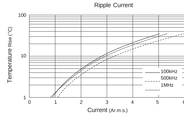
[Example of Temperature Rise (Heat Generation) in Chip Multilayer Ceramic Capacitors in Contrast to Ripple Current] Sample: R(R1) characteristics 10 \mu F, Rated voltage: DC10V
